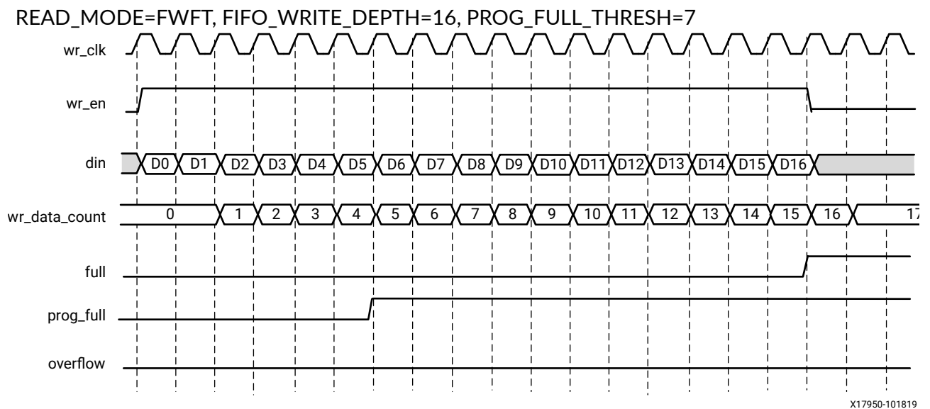
Figure 8: Write Operation
