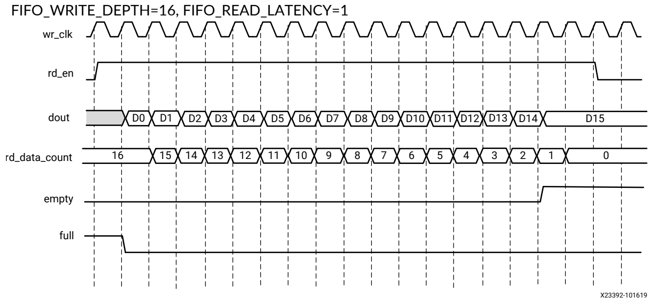
Figure 23: Standard Read Operation with Full Deassertion
