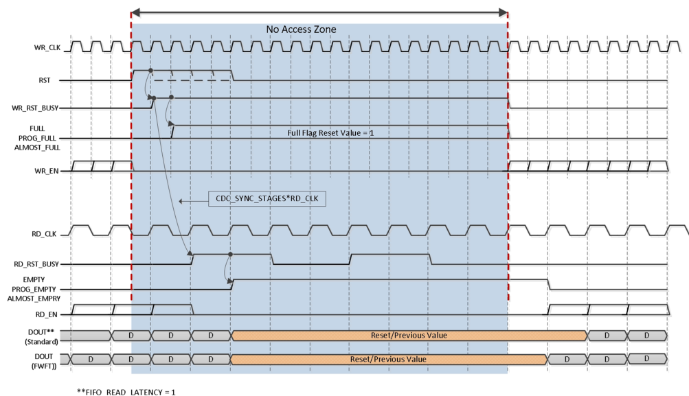
Figure 4: Reset Behavior
