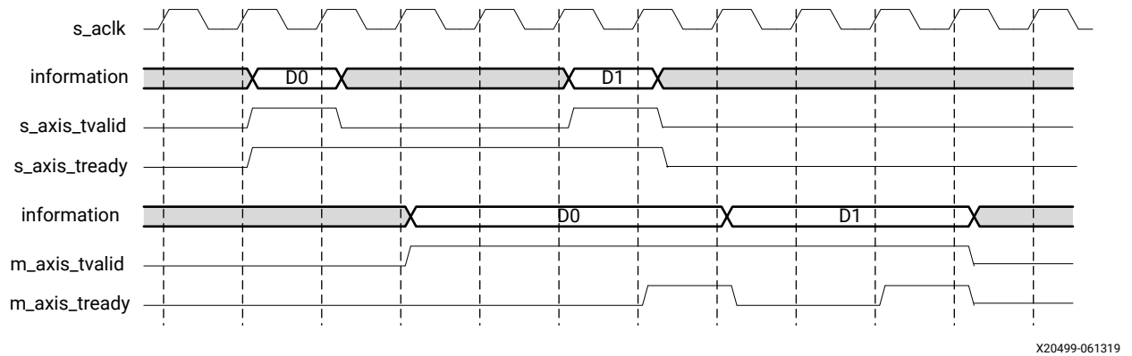
Figure 15: Timing for Read and Write Operations to the AXI Stream FIFO
