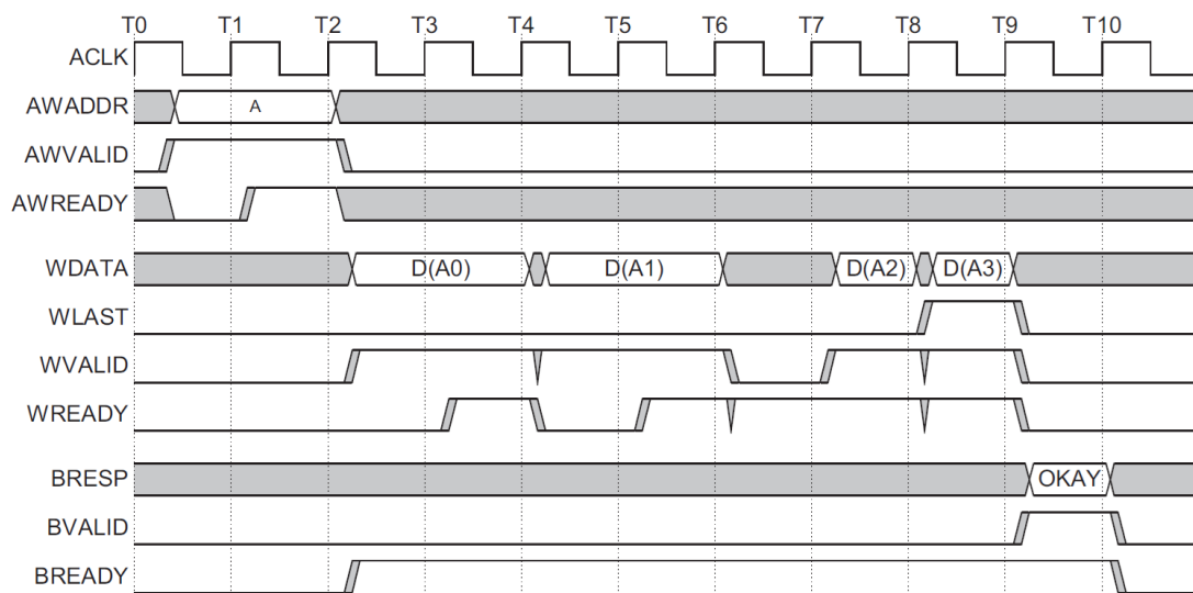
Figure 13: Timing Write Operations to the AXI4 FIFO
