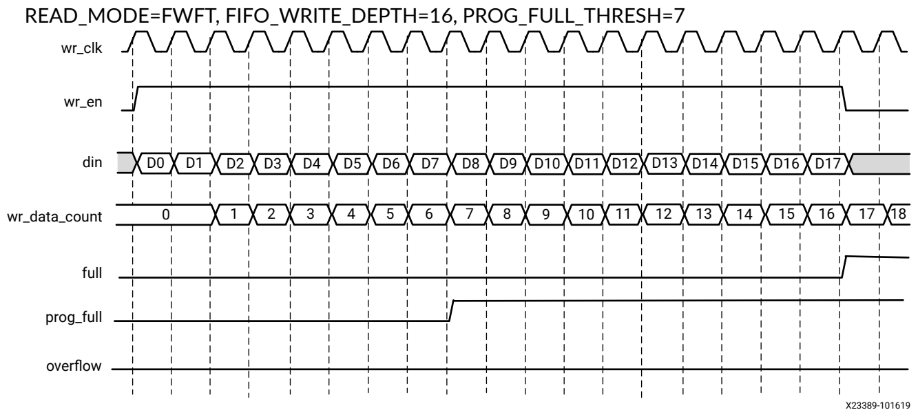
Figure 20: Write Operation
