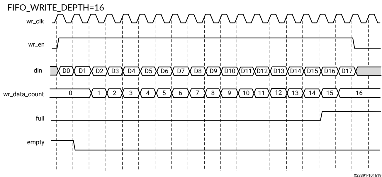
Figure 22: Standard Write Operation with Empty Deassertion
