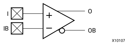
IBUFDS_DIFF_OUT
