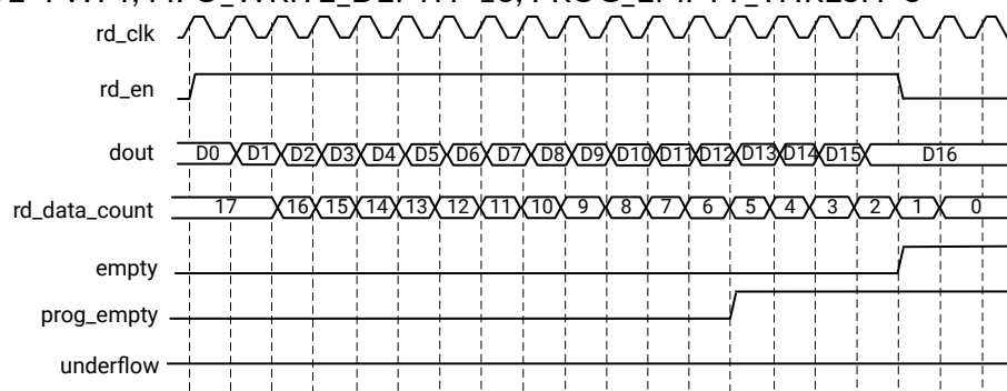
Figure 9: Read Operation
