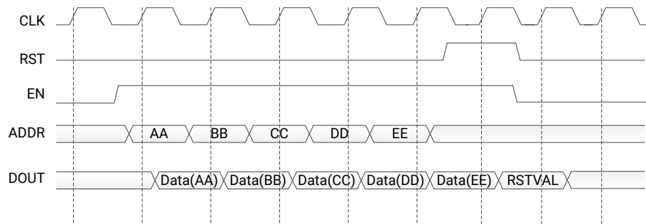
DPR0M with Read Latency of 2
