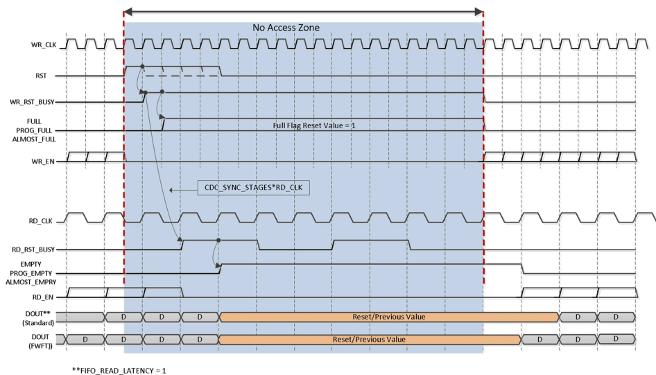
Figure 2: Reset Behavior
