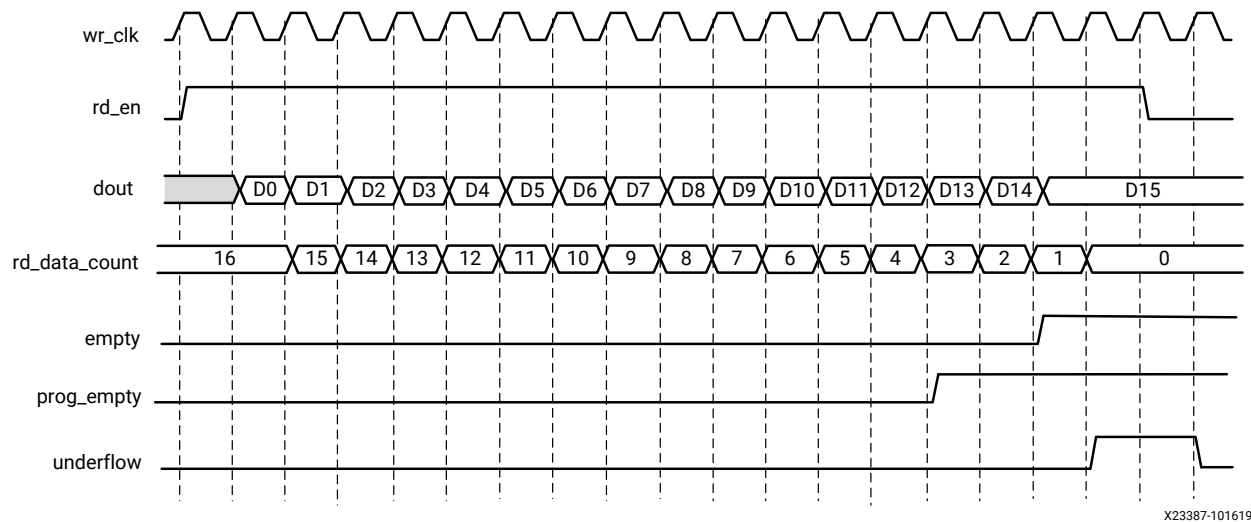
Figure 20: Standard Read Operation
