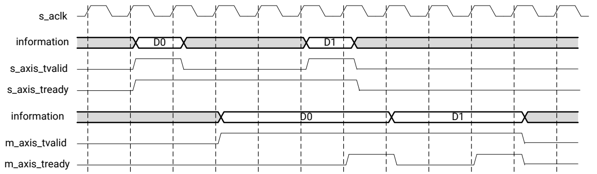
Figure 14: Timing for Read and Write Operations to the AXI Stream FIFO
