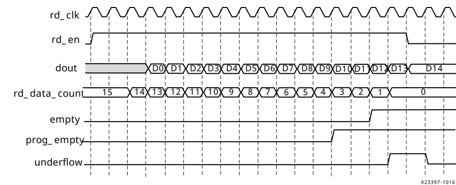
Figure 5: Standard Read Operation
