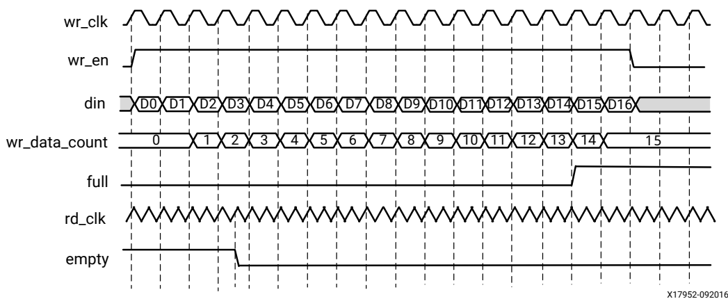
Figure 8: Standard Write Operation with Empty Deassertion
