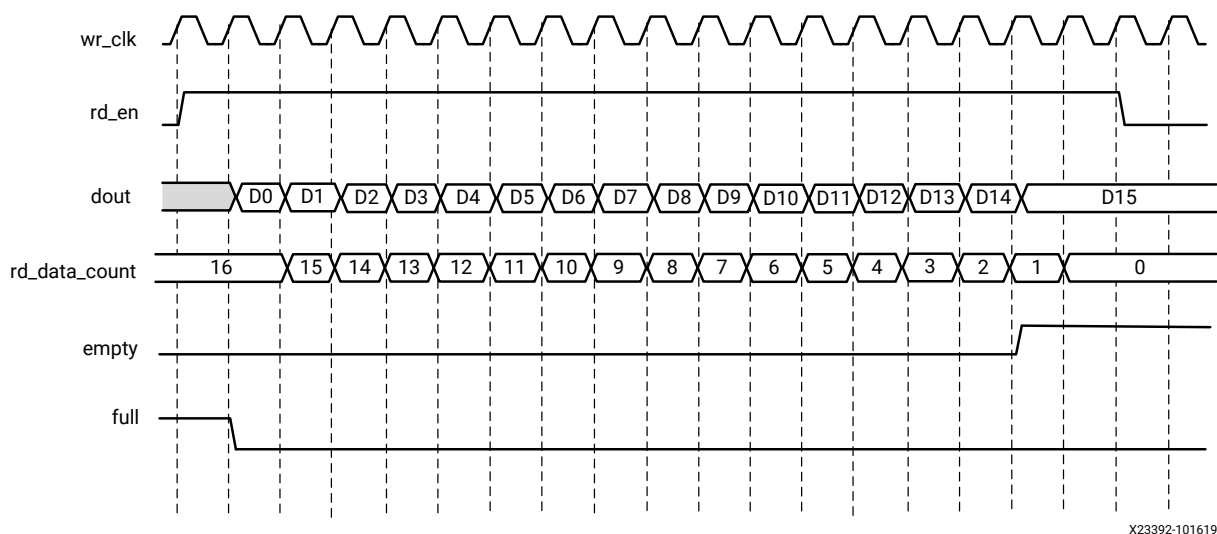
Figure 25: Standard Read Operation with Full Deassertion
