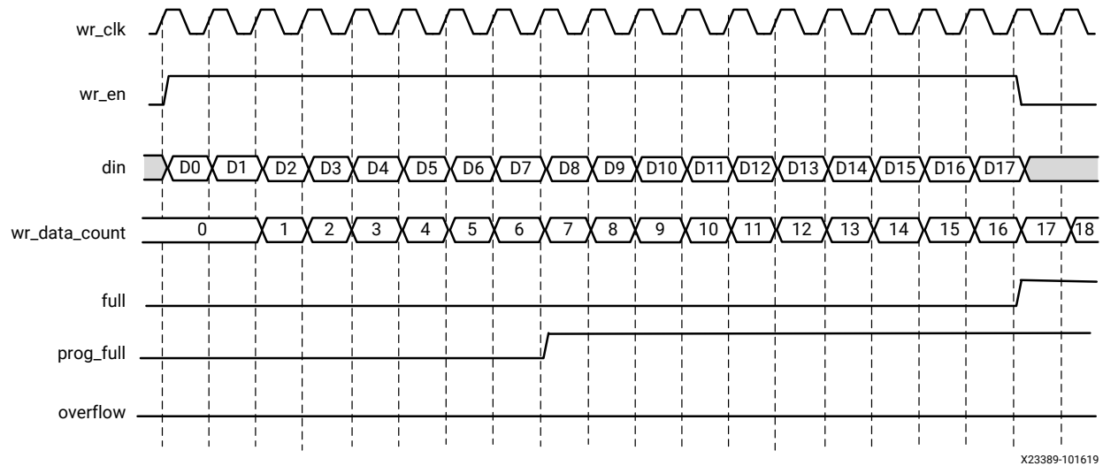
Figure 22: Write Operation
