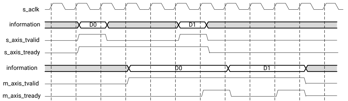
Figure 15: Timing for Read and Write Operations to the AXI Stream FIFO
