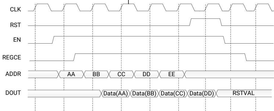
DPR0M with Read Latency of 2
