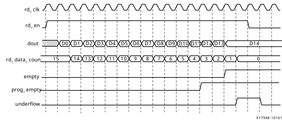
Figure 5: Standard Read Operation
