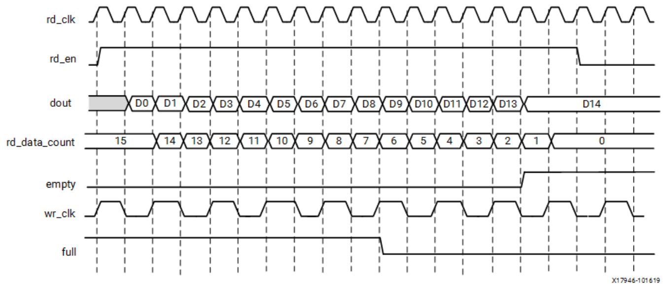
Figure 9: Standard Read Operation with Full Deassertion
