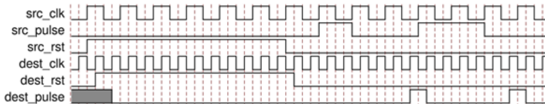
Figure 1: Timing for Macro and Transfer Back-to-Back Pulses
