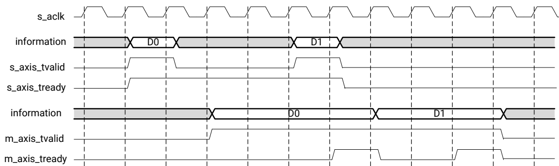
Figure 17: Timing for Read and Write Operations to the AXI Stream FIFO
