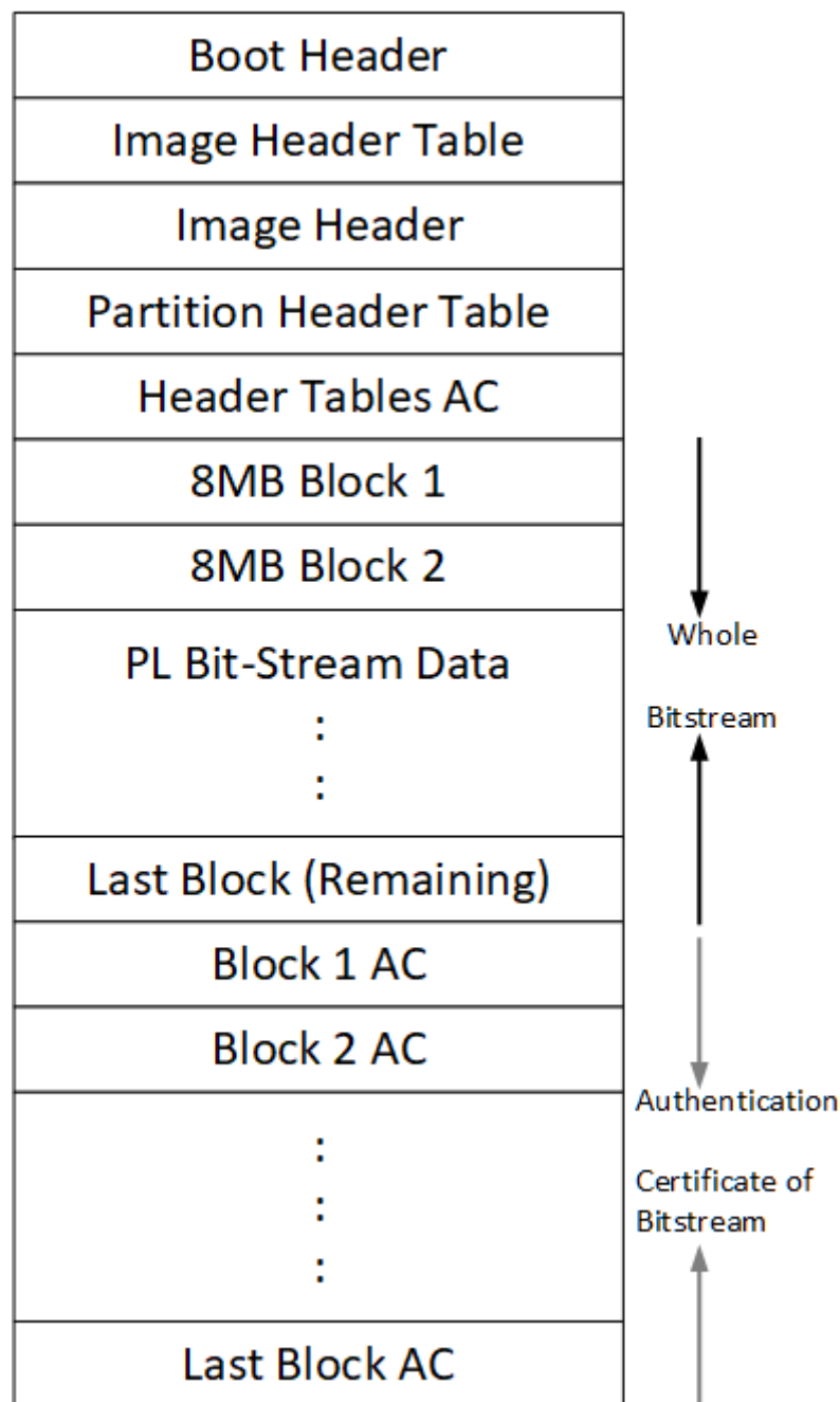
Figure 7: Bitstream Blocks
