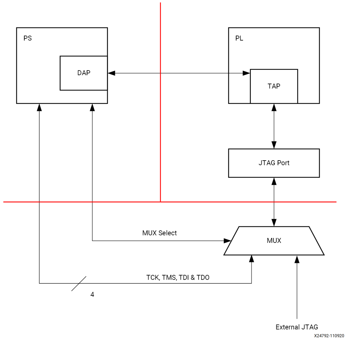
Figure 2: MUX Usage
