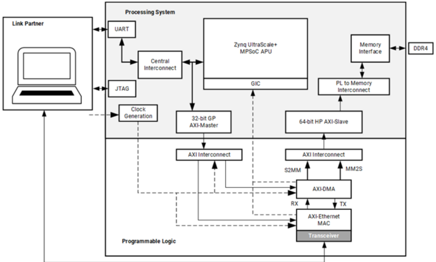
Figure 1: AXI Ethernet subsystem with DMA on Zynq Ultrascale+ MPSoC
