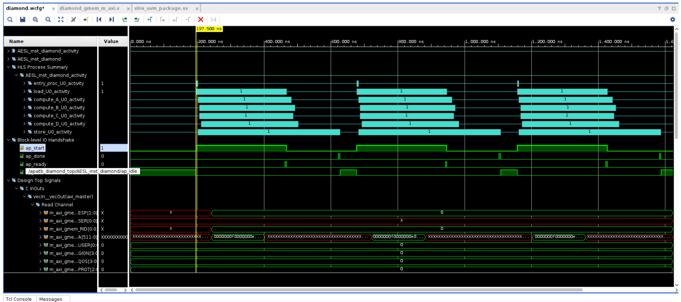
Figure 129: Waveform Viewer
