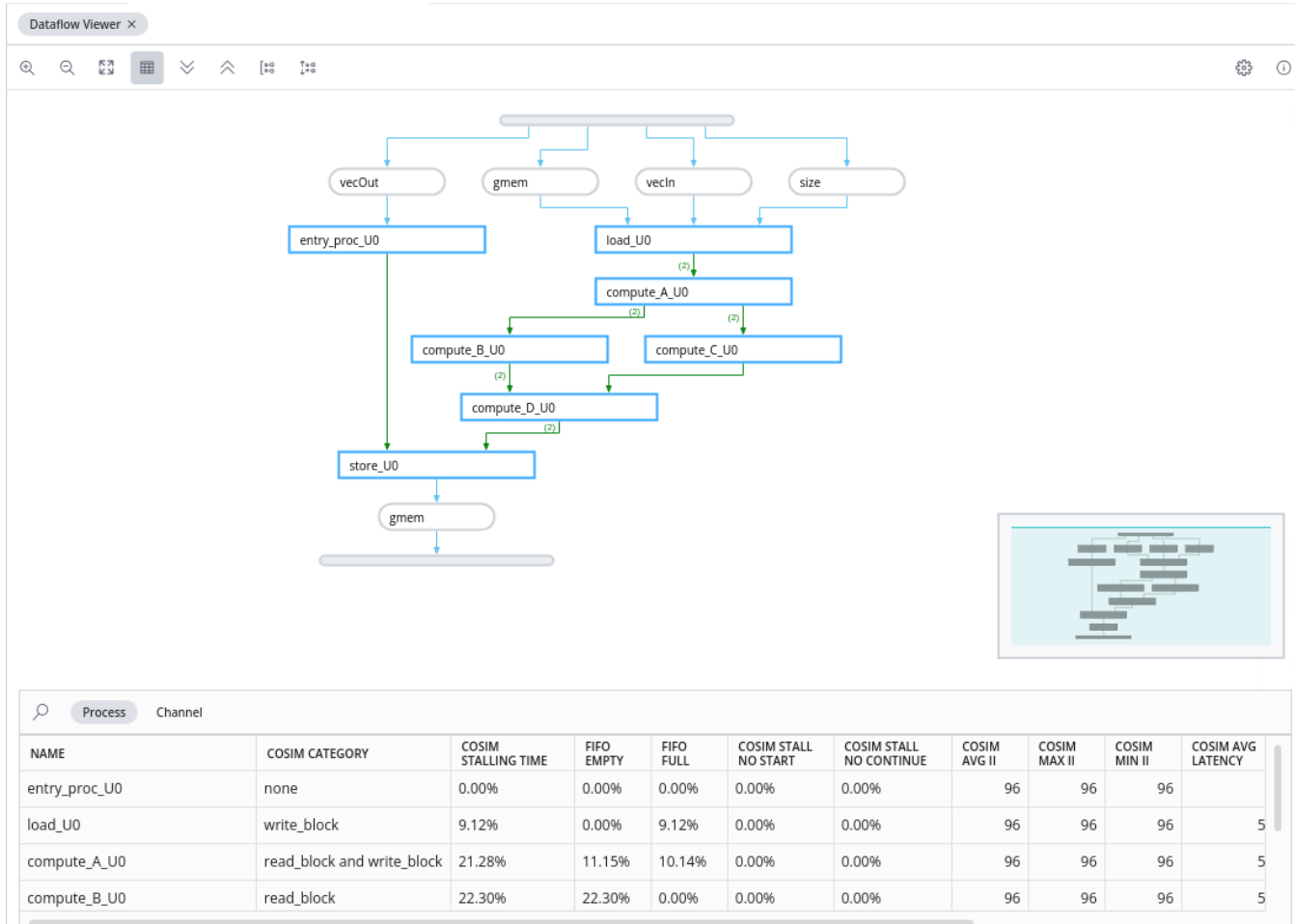
Figure 125: Dataflow Viewer
