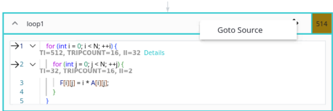
Figure 105: Graph View
