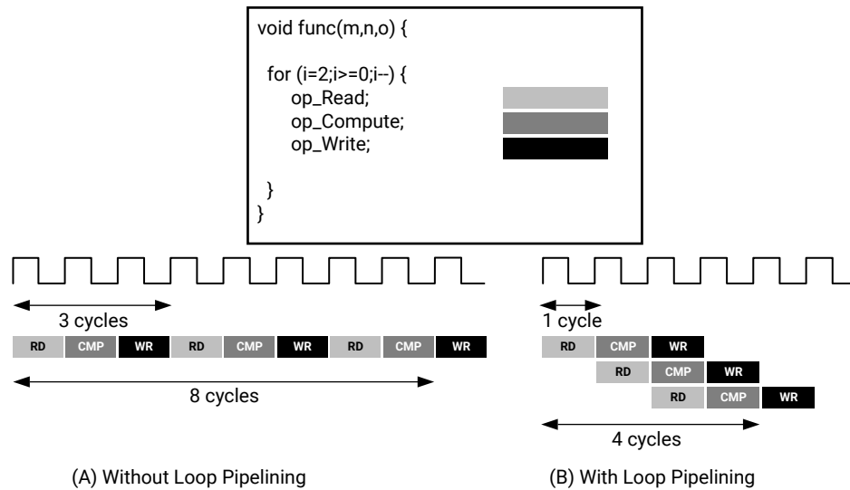
Figure 141: Loop Pipeline
