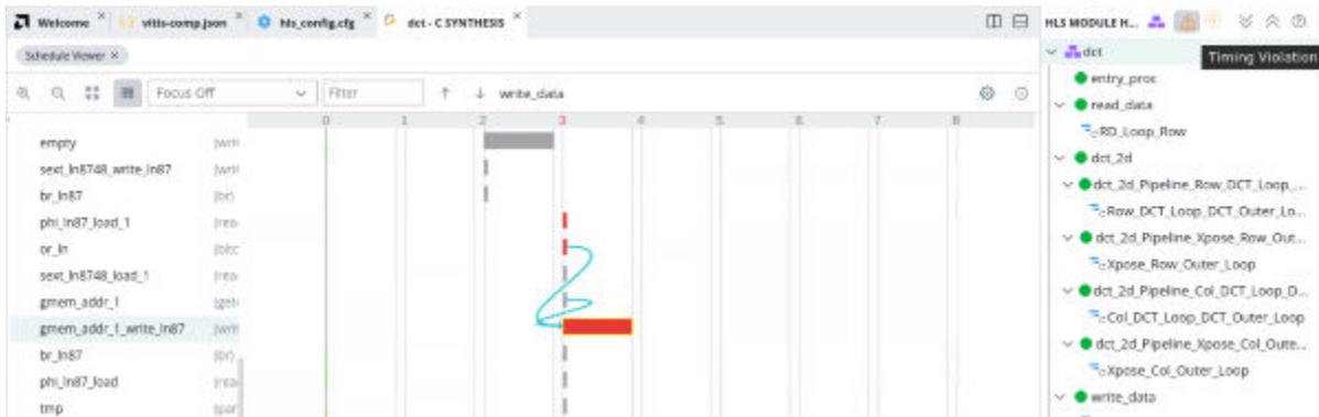
Figure 124: Timing Violations
