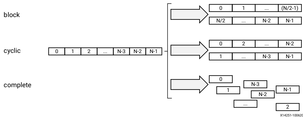
Figure 24: Array Partitioning
