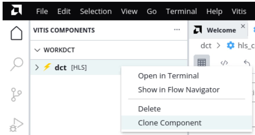
Figure 137: Clone Component
