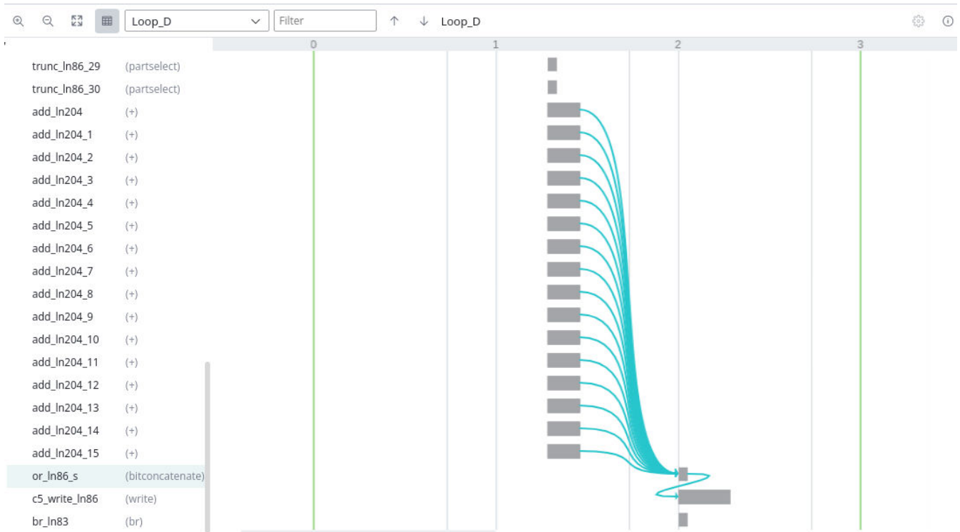
Figure 123: Pipelined Loop
