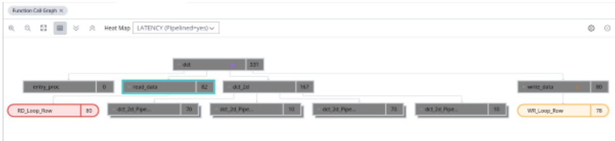
Figure 121: Performance Metrics
