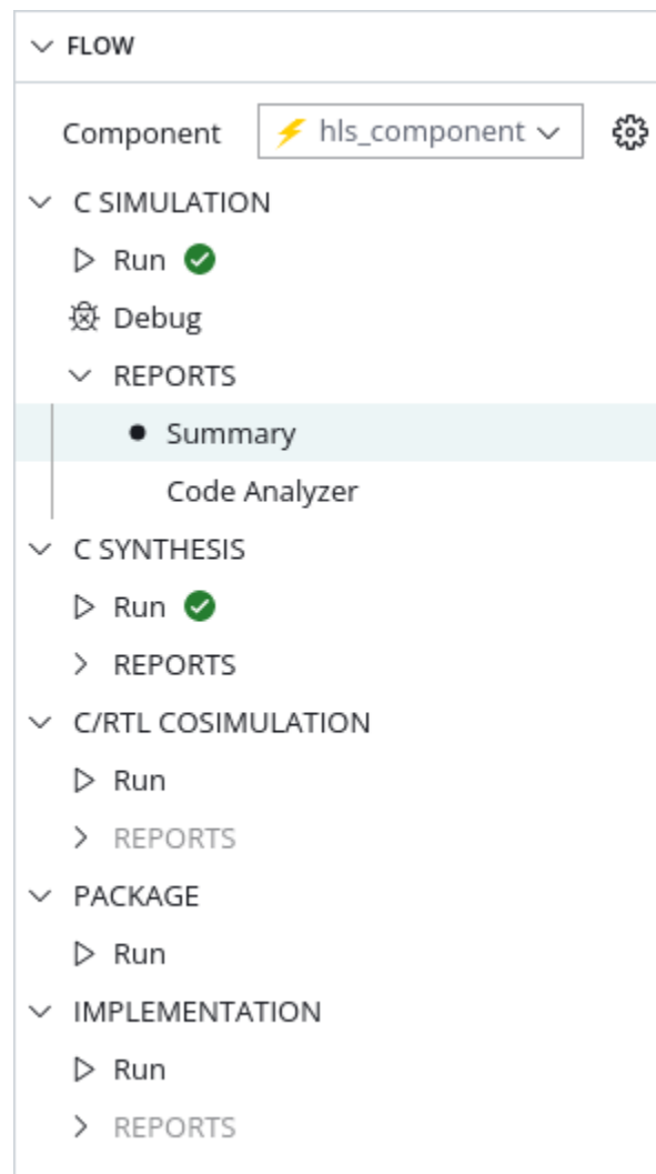
Figure 81: Flow Navigator
