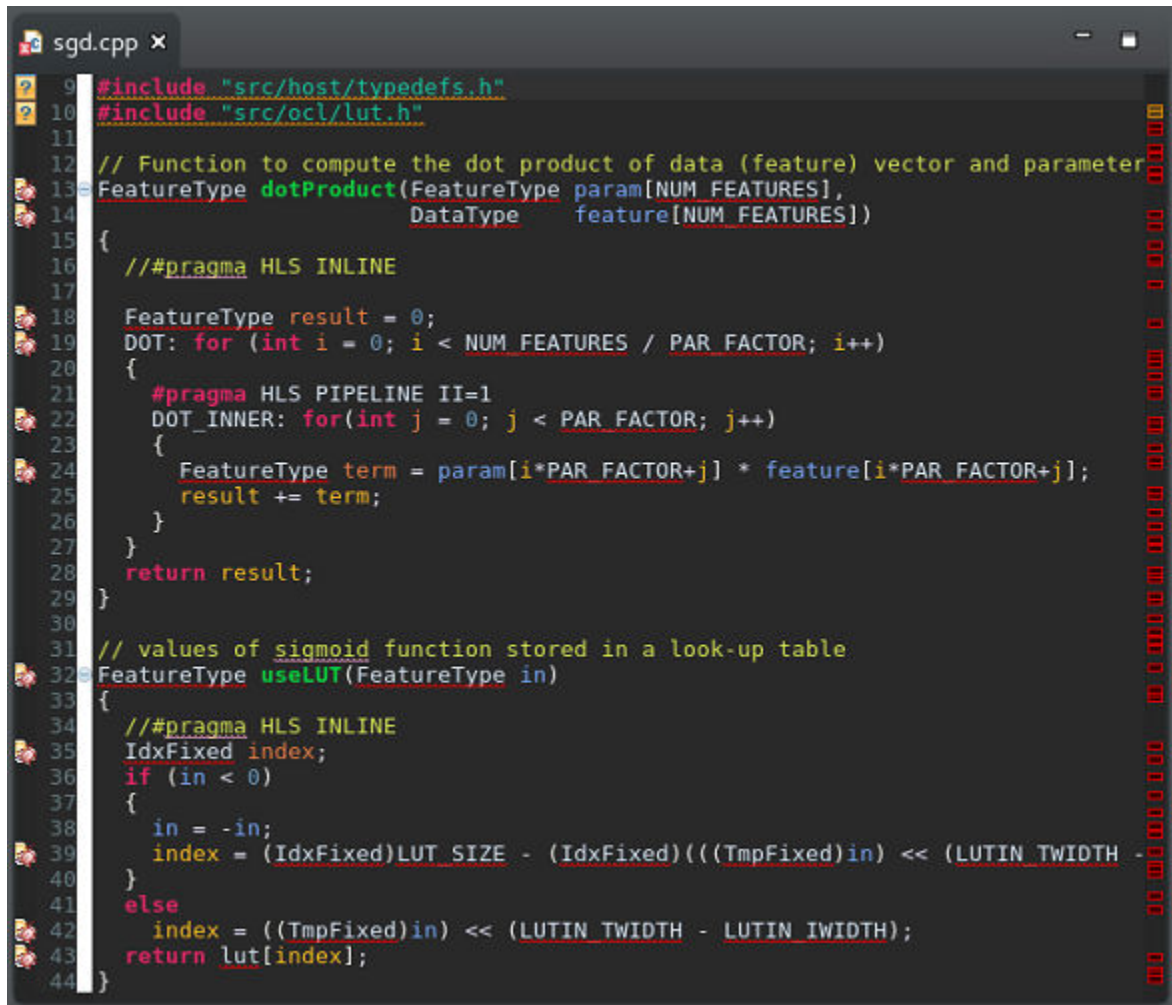
Figure 90: Unresolved References
