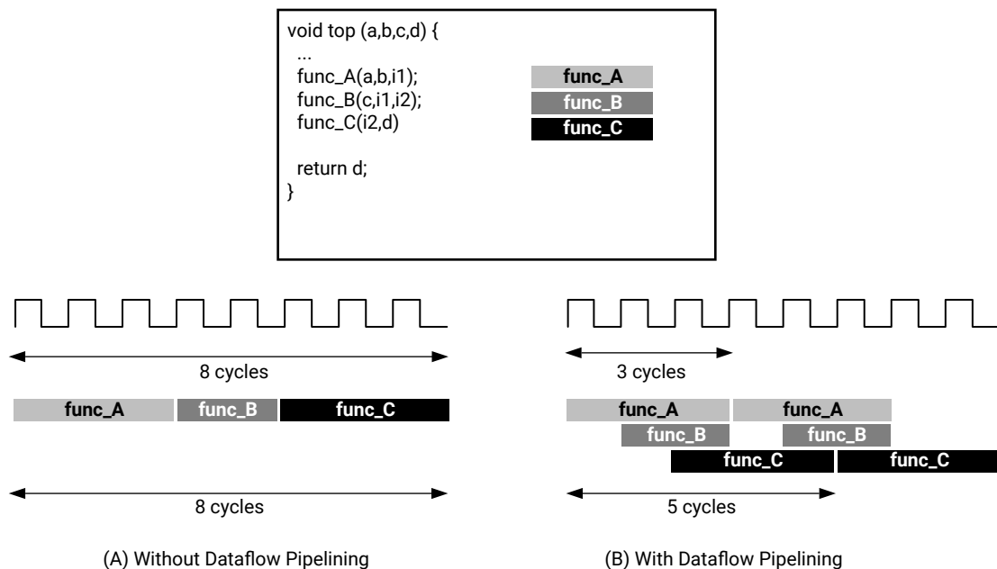
Figure 140: DATAFLOW Pragma
