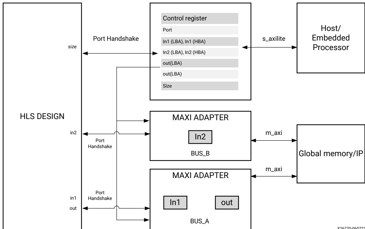
Figure 37: 2 MAXI Bundles
