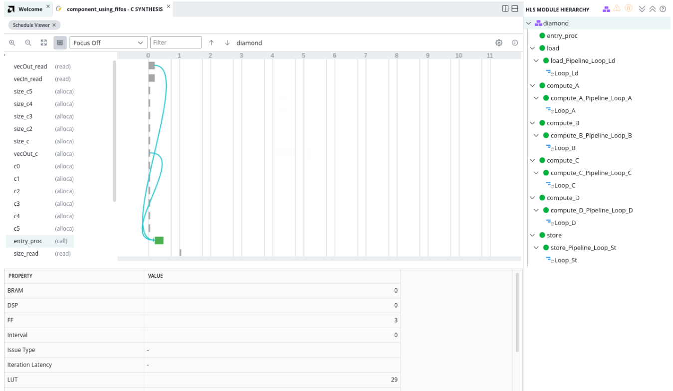
Figure 122: Schedule Viewer
