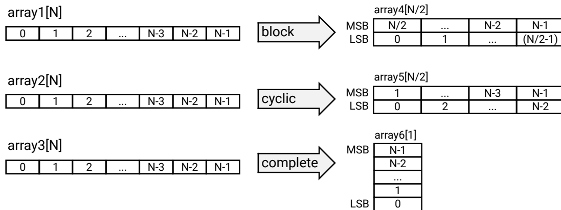
Figure 139: ARRAY_RESHAPE Pragma
