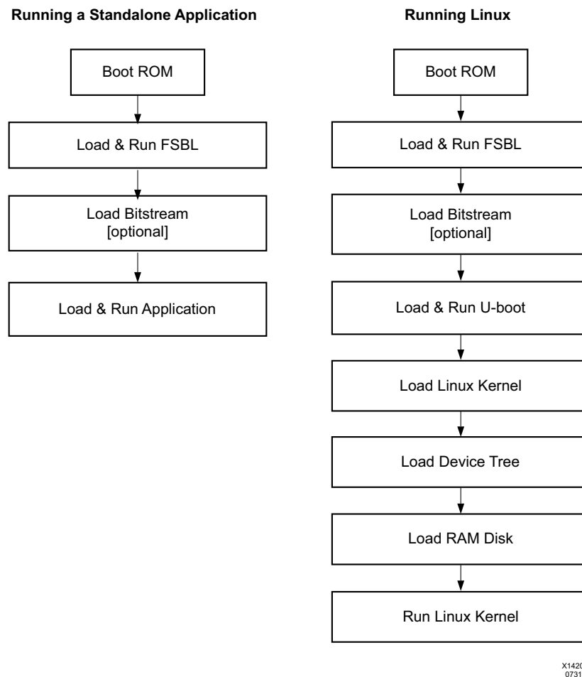
Figure 6-3: Boot Sequence and Boot Files
