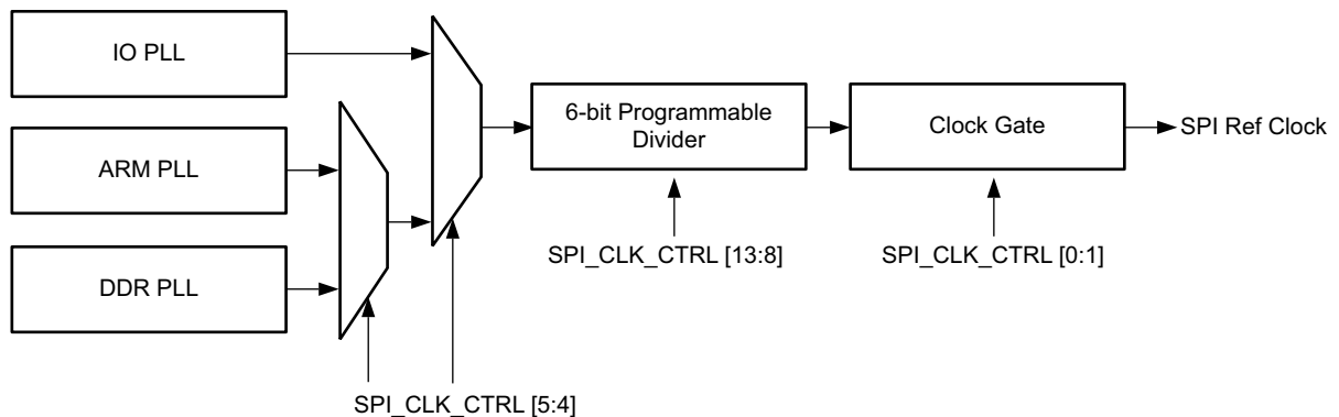
Figure 3-28: Clock Gating
