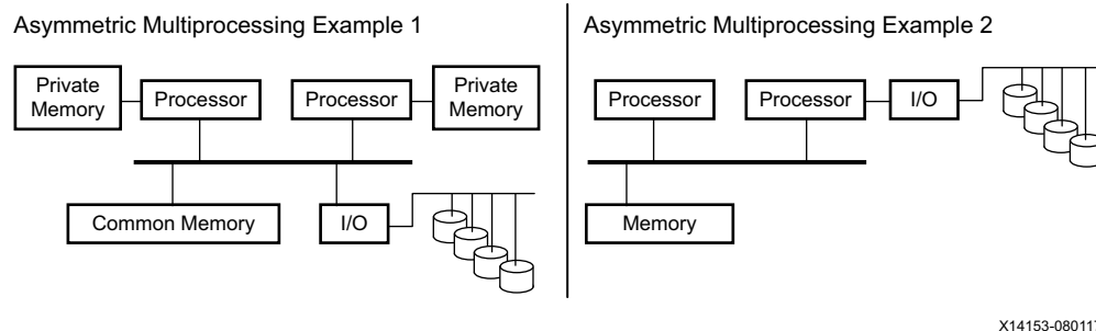
Figure 4-1: Typical AMP Configurations
