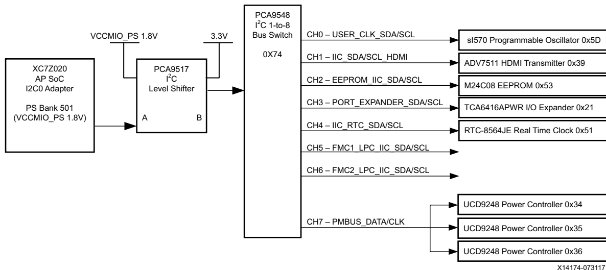
Figure 3-7: Example I2C Bus Topology
