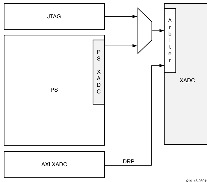
Figure 3-26: XADC Arbitration
