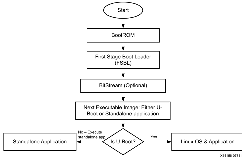
Figure 4-6: Boot Flow
