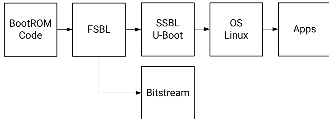
Figure 2: Secure Boot Chain of Trust
