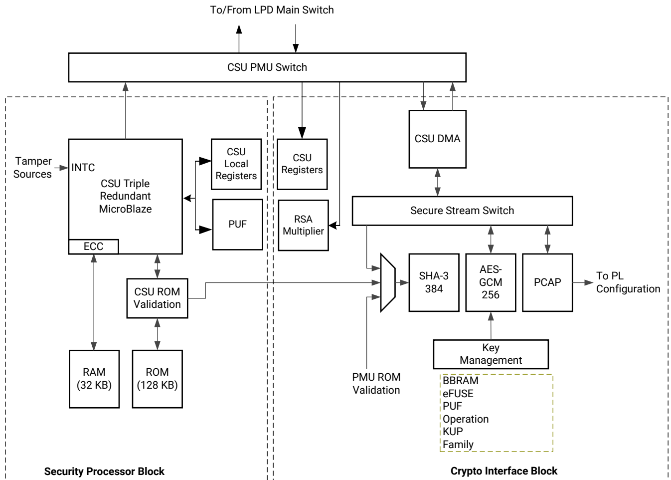
Figure 1: Configuration Security Unit Block Diagram
